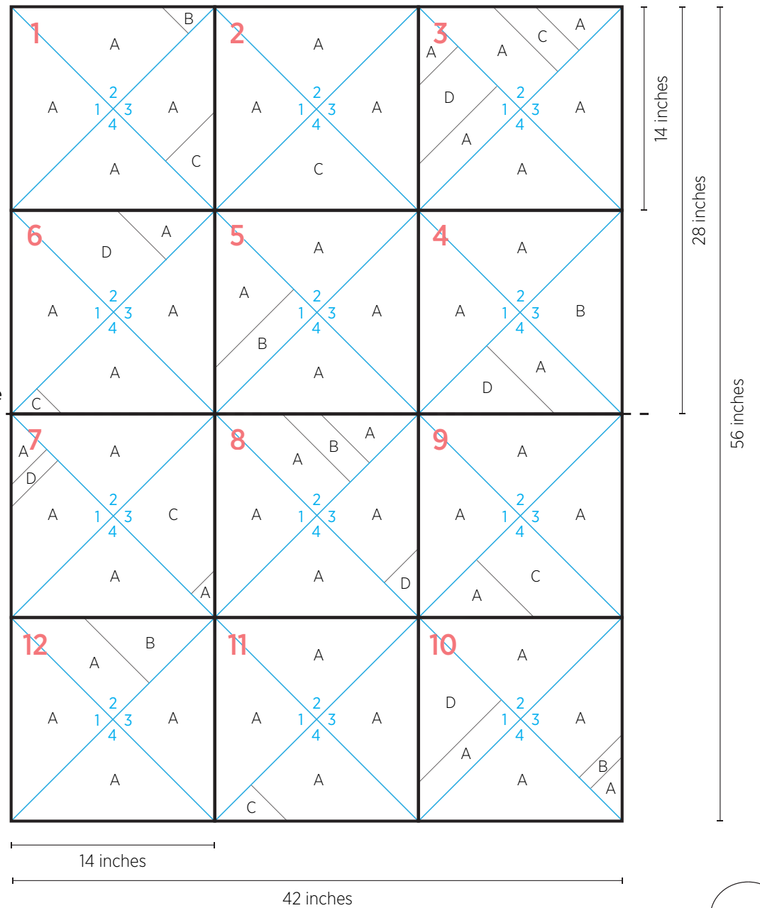
Layout Schematic
